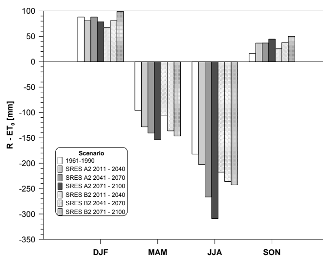
Fig. 1 Seasonal climate water balance in the period 1961–1990 and according to the climate change scenarios.
