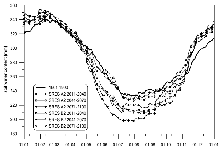
Fig. 2 Annual course of mean soil water content in the horizon 0–100 cm [mm] on Danubian Lowland in the period 1961–1990 and according to the climate change scenarios.
