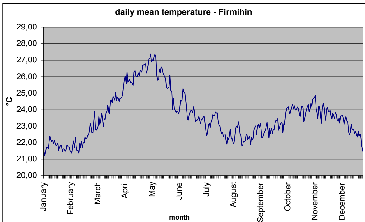
Fig. 5 – Daily means of temperature on Firmihin
