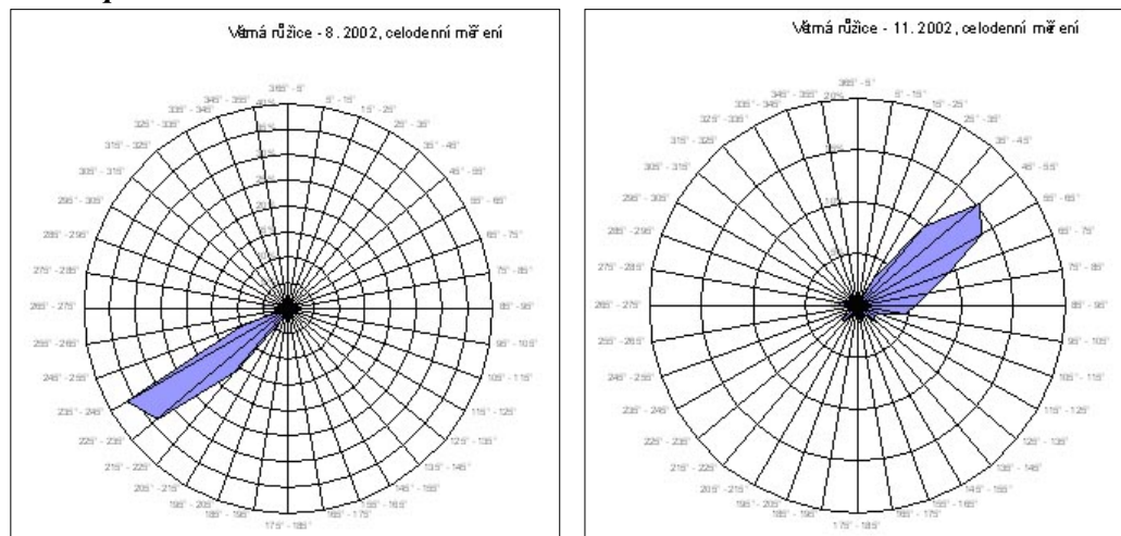
Fig. 7-8 – prevailing direction of winds during summer (left) and winter (right) monsoon (after Adolt 2001)
