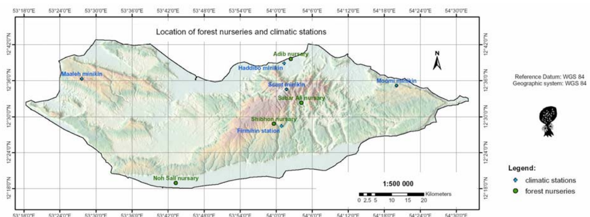
Fig. 2 – Location of weather stations on Soqatra
