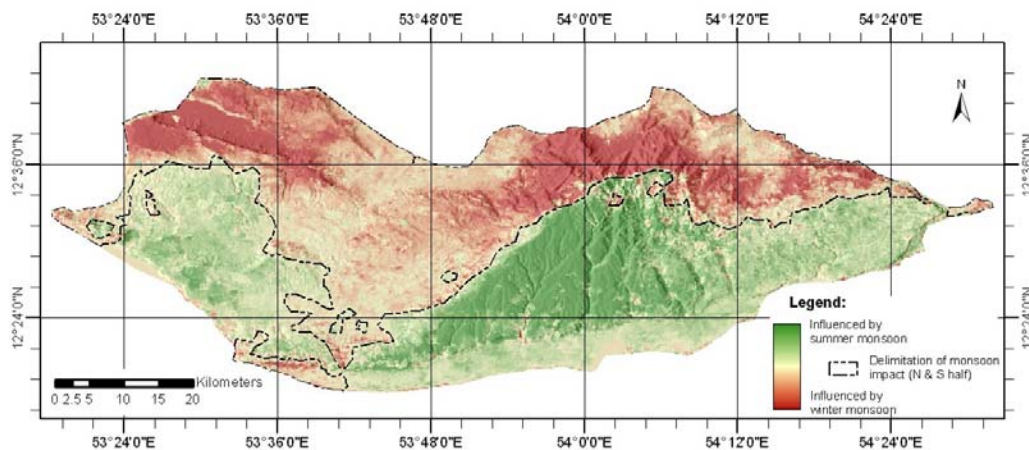
Fig. 3 – Impact of monsoons on different parts of the island
