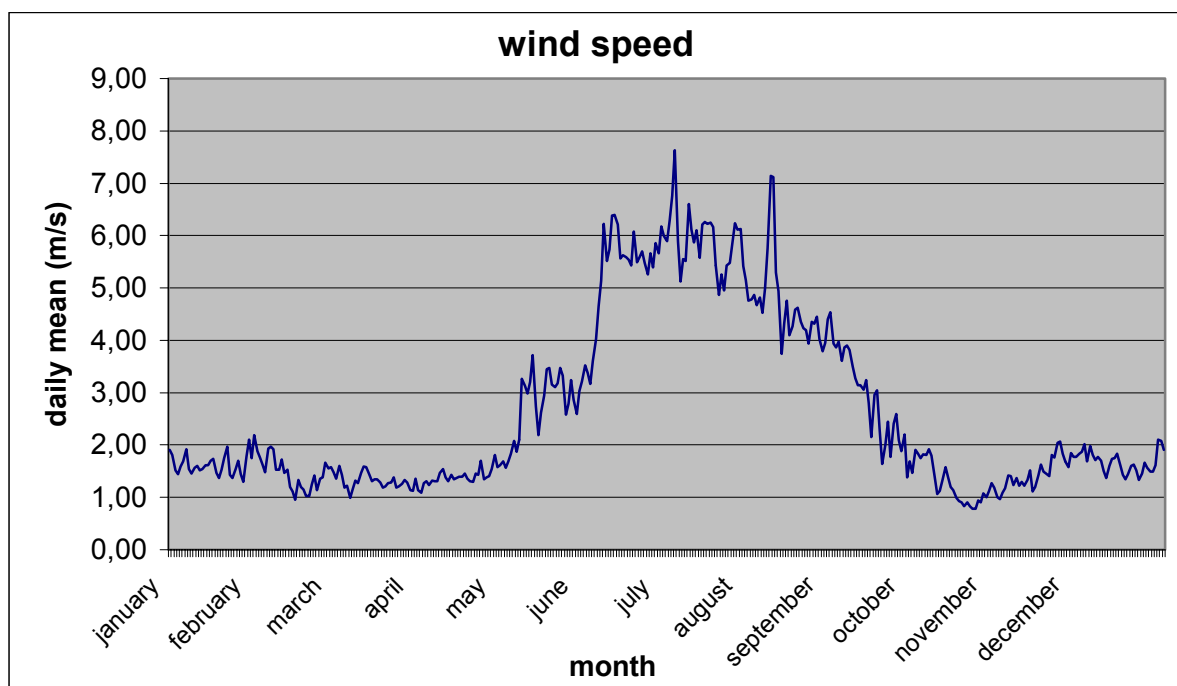
Fig. 9 – Daily means of wind speed on Firmihin in 2002
