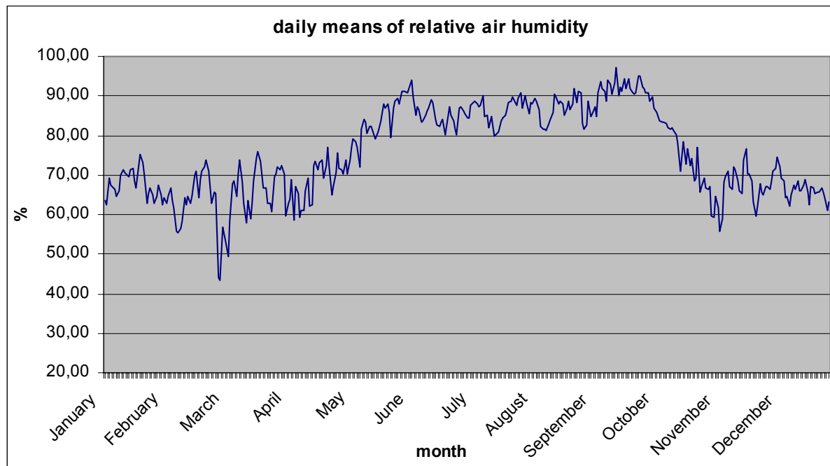
Fig. 6 – Daily means of relative air humidity on Firmihin
