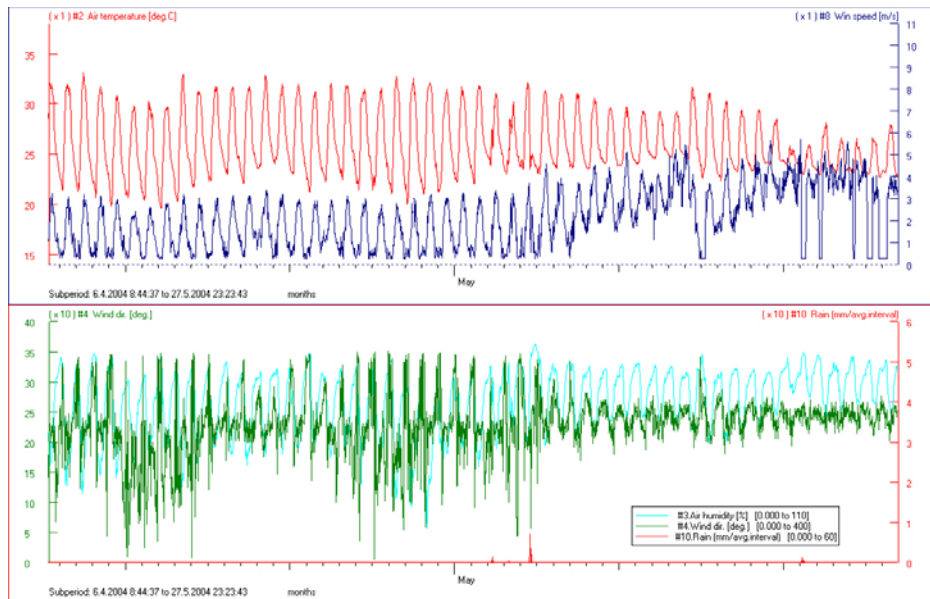
Fig. 4 - Example of start of summer monsoon in 2004
